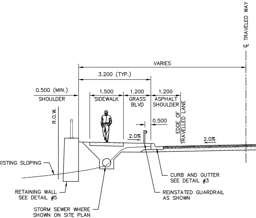
SECTION A-A TYPICAL CROSS SECTION NOT TO SCALE
